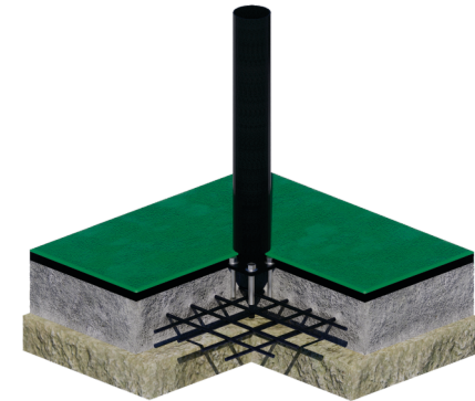
CONCRETE+RUBBER ANCHORAGE
