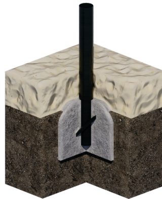
CONCRETE+SAND ANCHORAGE
